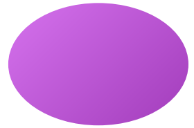
ellipse()
